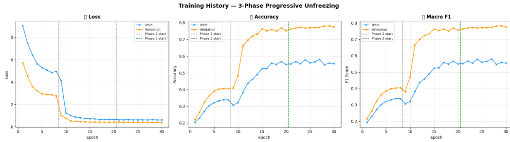
Figure 1: Training loss, accuracy, and macro F1-score across three training phases.
